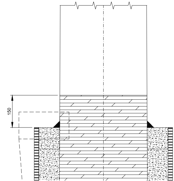
WATER PROOFING Scale 1:10
