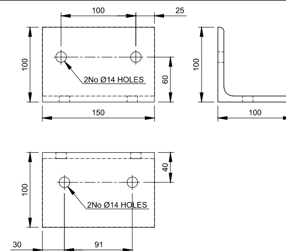
TPL-D - EA100x100x8 Scale 1:5
