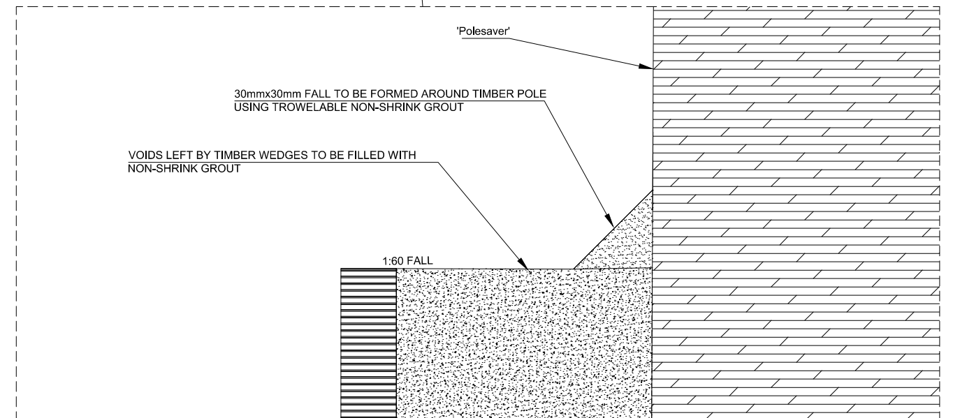
ENLARGED DETAIL Scale 1:2
