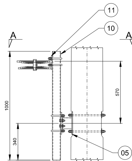
DETAIL H - Rx ANTENNA MOUNT Scale 1:20
