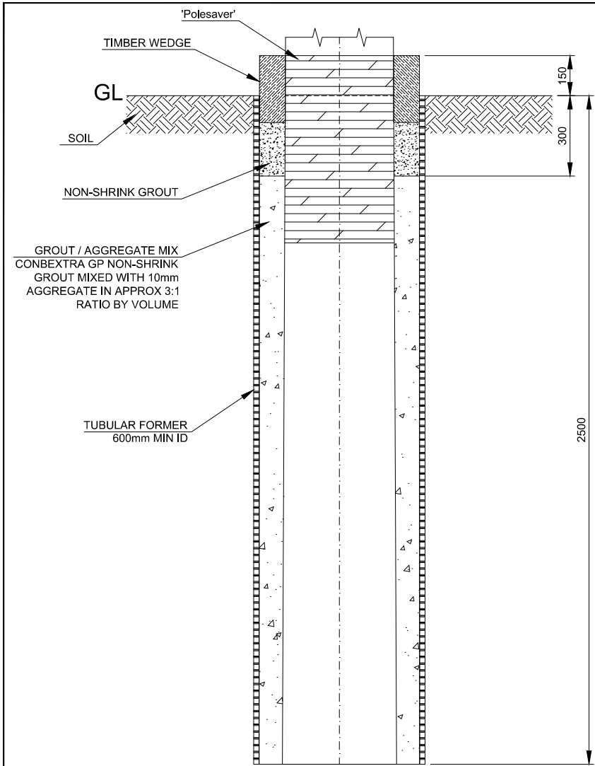
POROPOSED INSTALLATION ELEVATION Scale 1:20
