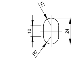
SLOTTED HOLE DETAIL Scale 1:2
